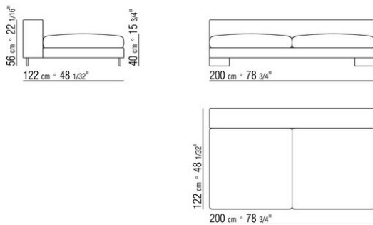
COD. 011P11 ELEMENT / DACRON
