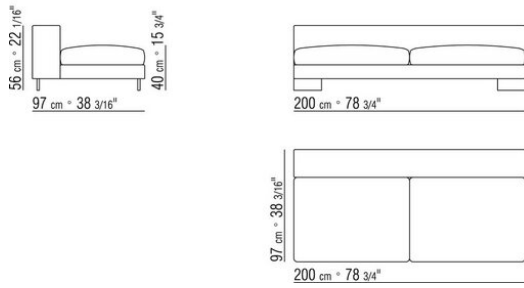
COD. 011P15 ELEMENT / DACRON
