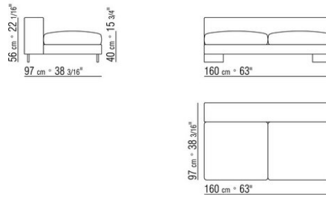
COD. 011P04 ELEMENT
