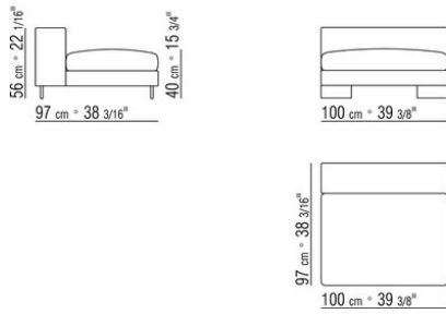
COD. 011P03 ELEMENT
