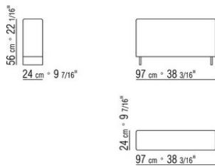
COD. 011P72 ARMLEHNE KERNLEDER
