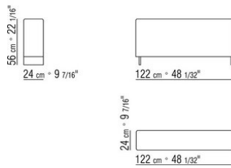
COD. 011P73 ARMLEHNE KERNLEDER
