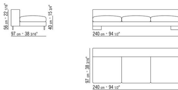
COD. 011P06 ELEMENT
