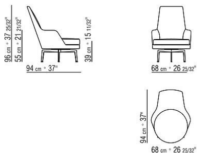
COD. 015M13 GA.13-SESSEL HOLZGESTELL FIX
