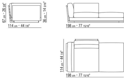
COD. 014V31 ECKELEM L RUEC/ARM GEPLSTER
