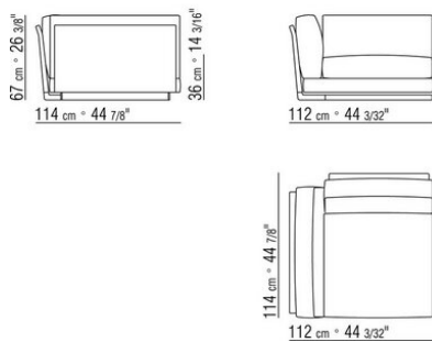
COD. 014V41 SOFA / ECKELEM RUECK ARM KERNLEDER
